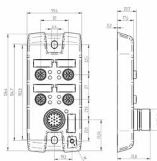
ASBS-R/ASBS-R... LED
